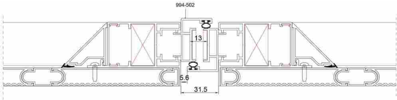
Section A Scale 3:4
