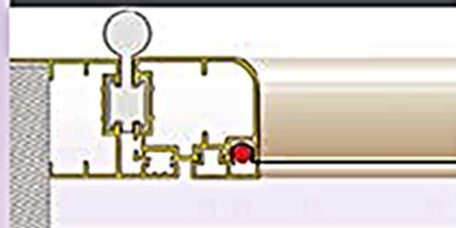
MARCO PERFIL EN "Z" A SOLICITAR FRAME PROFILE "Z" UPON REQUEST
